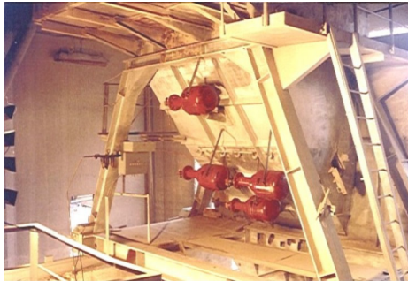
CLINKER Cuptor de calcinare HEIDELBERG CEMENT GROUP CARPATCEMENT-FIENI-ROMANIA
